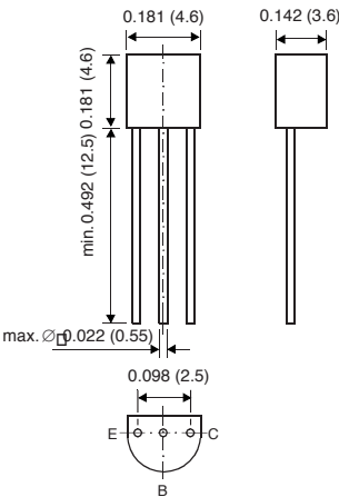
TO-92
